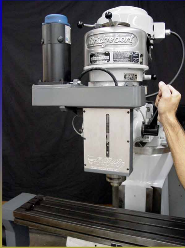
Elrod Patented Z Axis Quill Drive with Quick Disconnect
